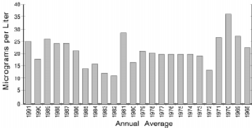
Above: Concentrations of arsenic at the DWP's Sylmar filtration plant from 1968 to 1991 lie well below the current drinking-water standard of 50 micrograms per liter. If that standard drops to 2–20 \mu\text{g/l} , however, there will be trouble meeting it.
